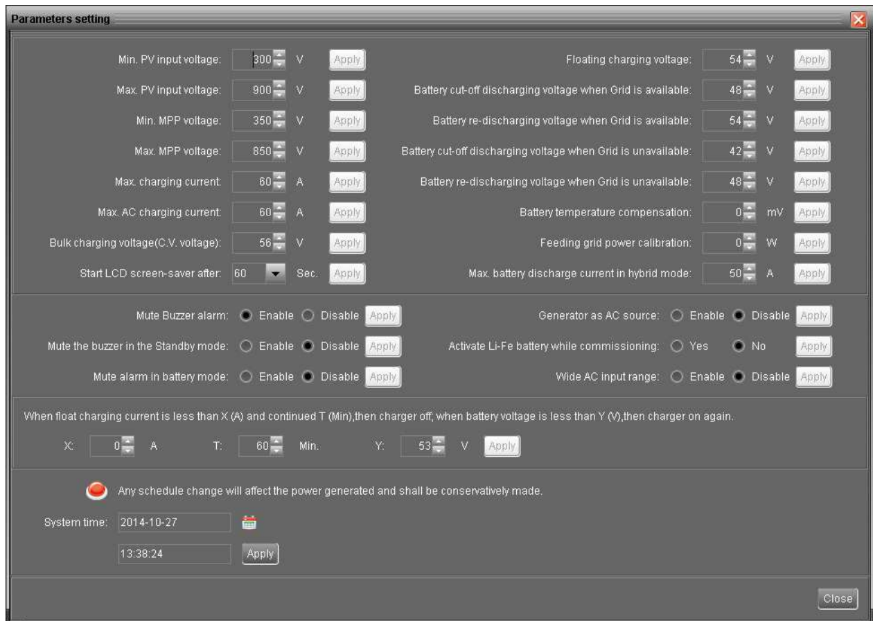
Diagram 4-11C (Off-Grid mode)
