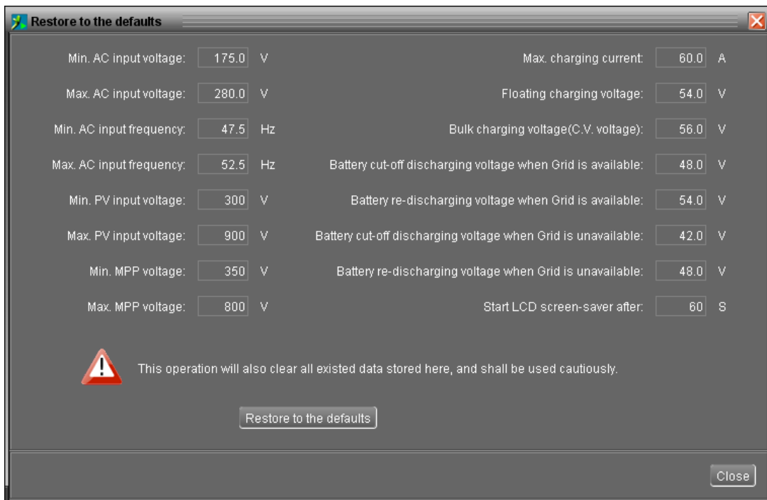
Diagram 4-12B (Off-Grid)
