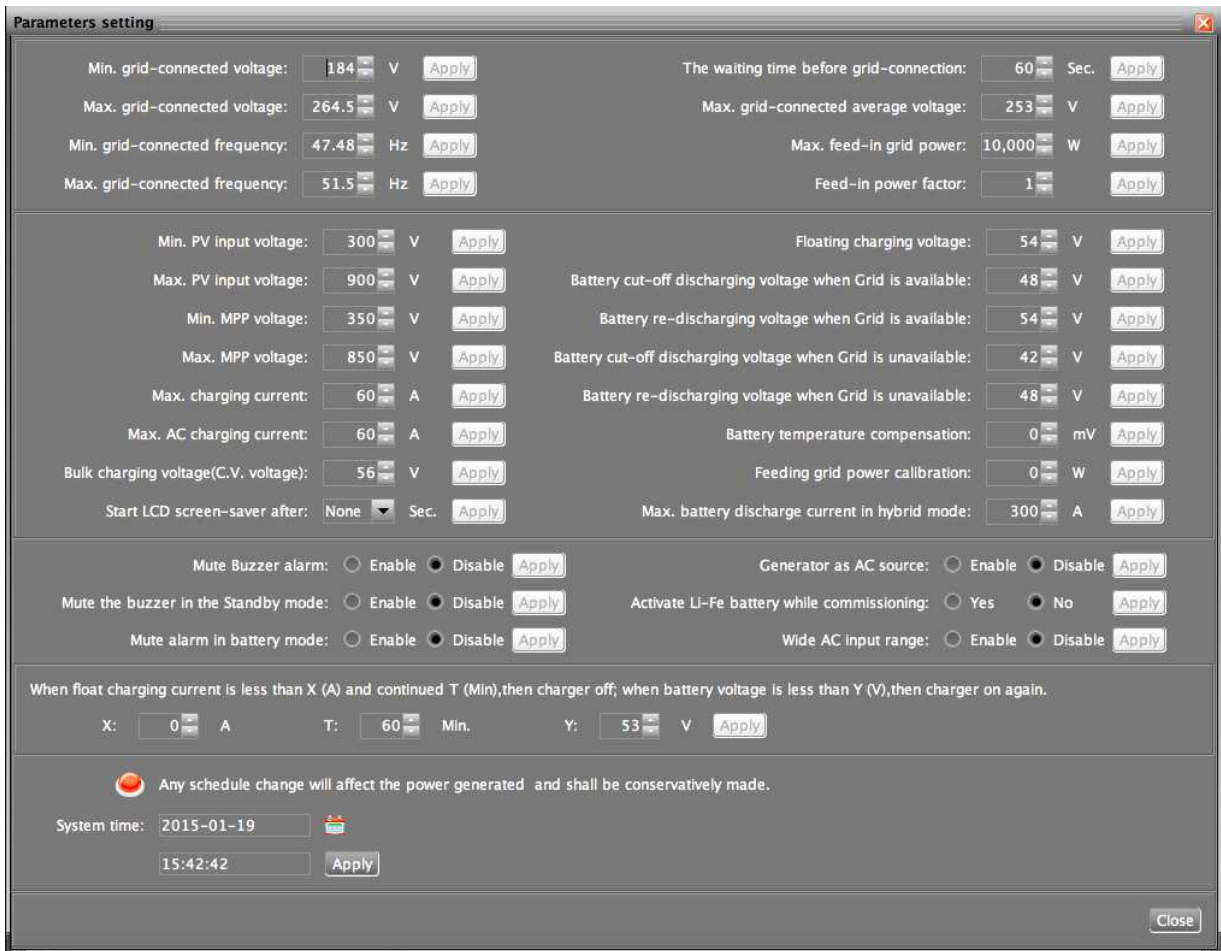
Diagram 4-11A (Grid-Tie with Backup mode)
